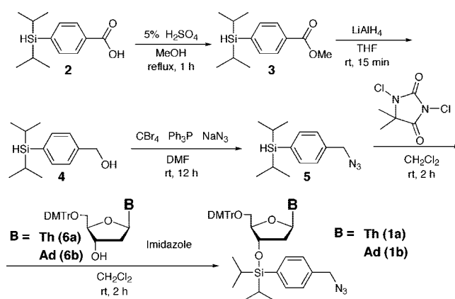
FIGURE 1. Skeletons of previous N-protected loading reagents and loading reagents 1a–d containing a silyl linker without base protection.
